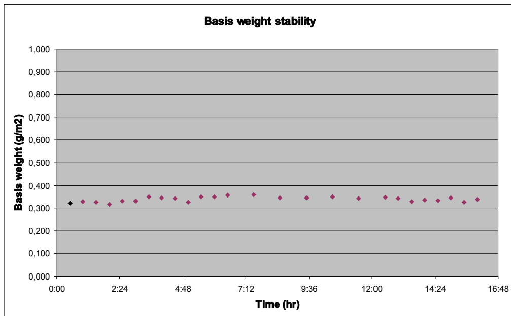
Figure 9. Consistency of nanofiber layer basis weight produced with industrial nozzle-less electrospinning equipment
