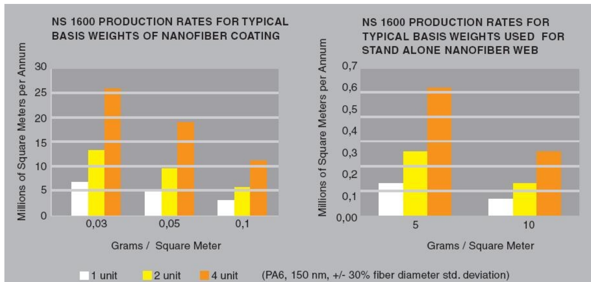
Figure 11. Production capacity of the nozzle-less electrospinning line with Polyamide 6
