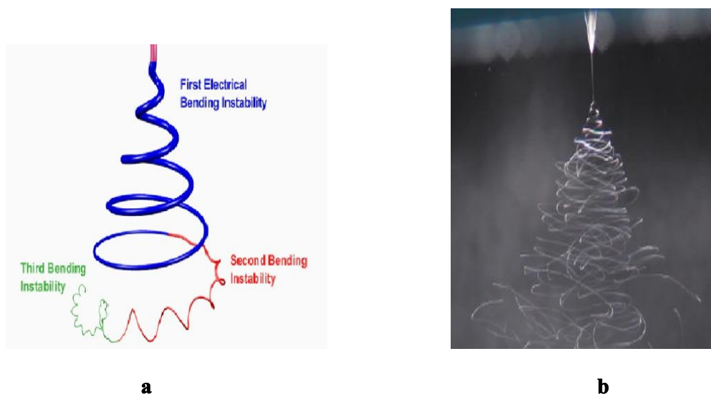
Figure 1. The path of an electrospinning jet (a – schematic, b – stroboscopic photograph). (Courtesy of Darrell Reneker, University of Akron)
