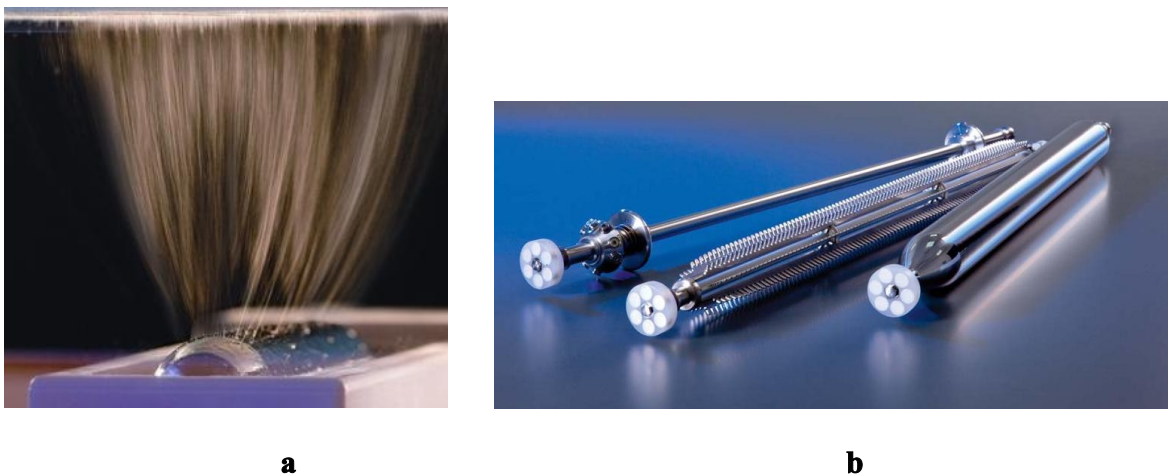
Figure 5. Free liquid surface electrospinning from a rotating electrode (a) and various types of spinning electrodes (b)
