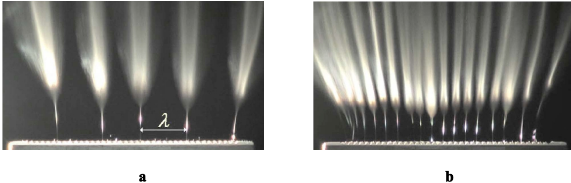
Figure 4. Free liquid surface electrospinning of Polyvinylalcohol at 32 kV (a) and 43 kV (b) (Courtesy of David Lukas, Technical University of Liberec)
